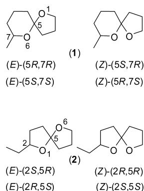
Figure 1. Chemical structures showing the relative cis/trans configurations, possible stereoisomers, and pertinent numbering for conophthorin, 7-methyl-1,6-dioxaspiro[4.5]decane, 1 , and chalcogran, 2-ethyl-1,6-dioxaspiro[4.4]nonane, 2 .
